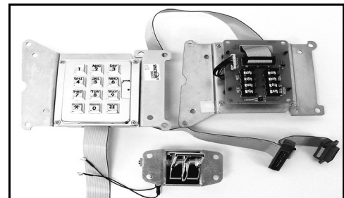
SP5130 Protel® Spectrum™ Armor Keypad
