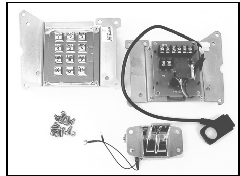
SP5110 2 pc Elcotel® Spectrum™ Armor Key-
