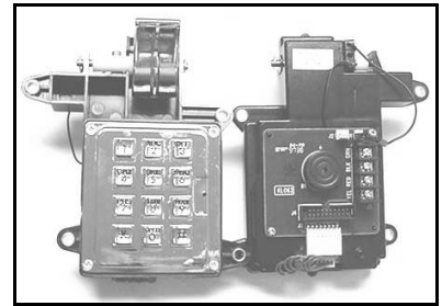
AE009 Intellicall Cost saver Keypad
