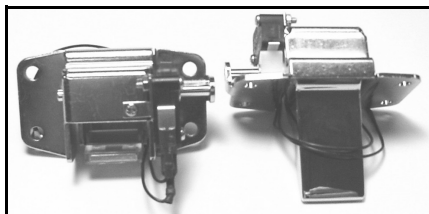
CL111 ARMORED HOOKSWITCH W/ MAGNETIC AND MICROSWITCHES
