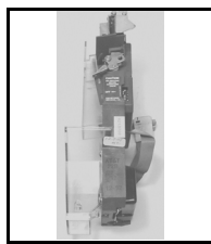
WE402 22B Coin Mechanism
